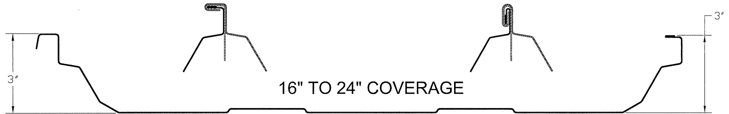
MODEL TSS-3000A 3" TRAPEZOIDAL STANDING SEAM UL 580 CLASS 90
