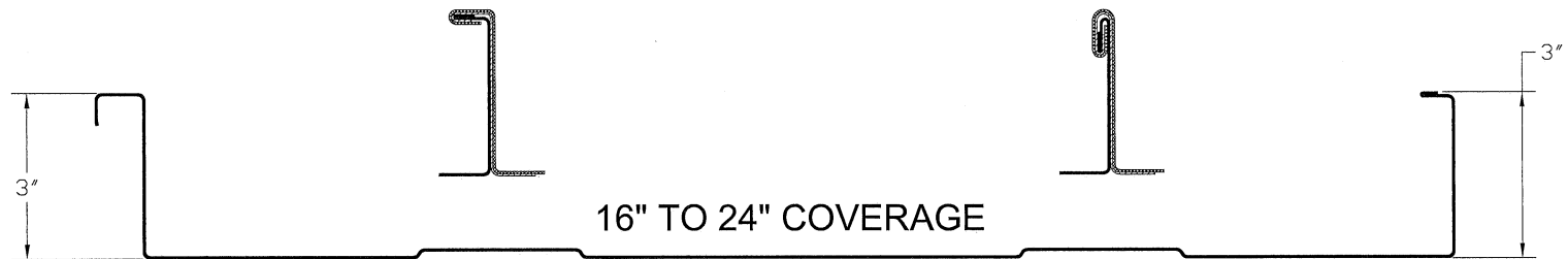
MODEL SS-3000 3" STANDING SEAM
